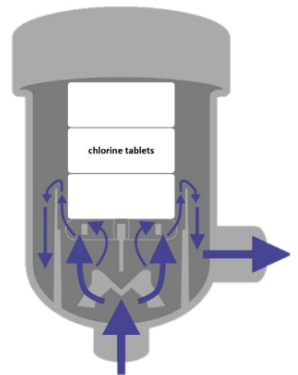
Cross-sectional View of Water Mission's Erosion Chlorinator
